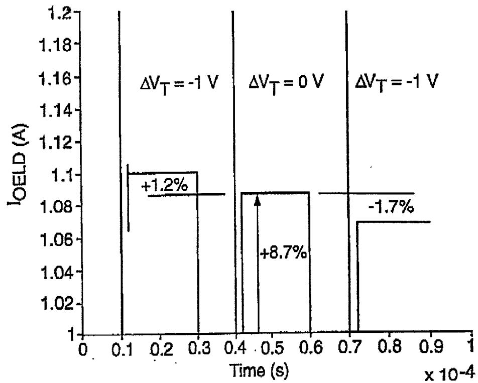
Fig.10. \times 10^{-6} Magnified I_{OELD} Response
